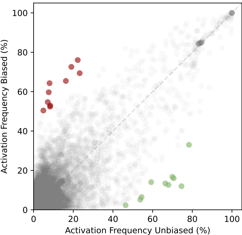
Activation Frequencies of SAE Latents: Stereoset
